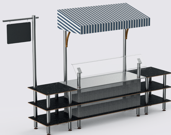
CLASSIC CANOPY STATION STATION CLASSIC CANOPY L 330 CM B 85 CM H 243,5 CM
